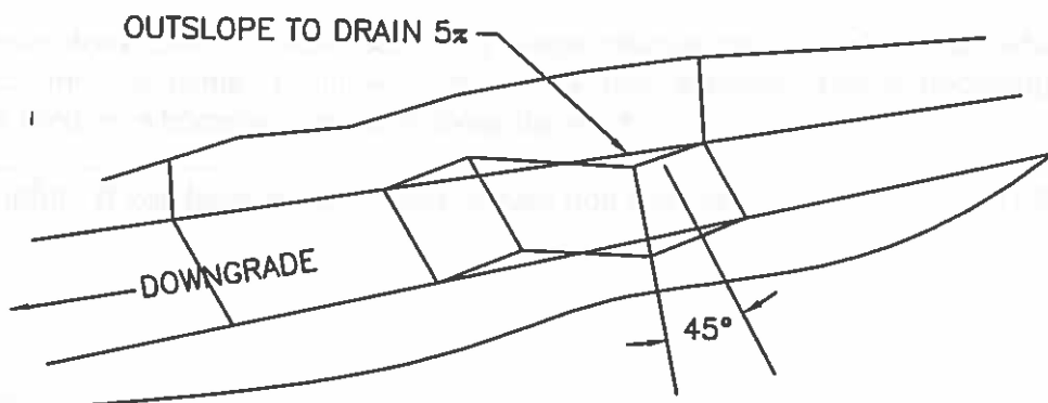
PERSPECTIVE VIEW
